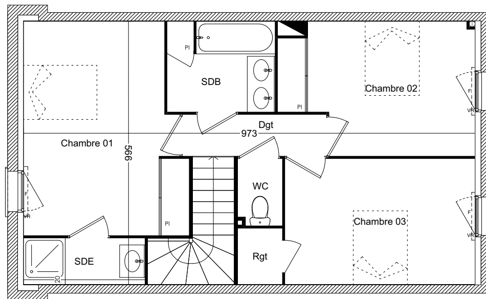
Plan R+1
