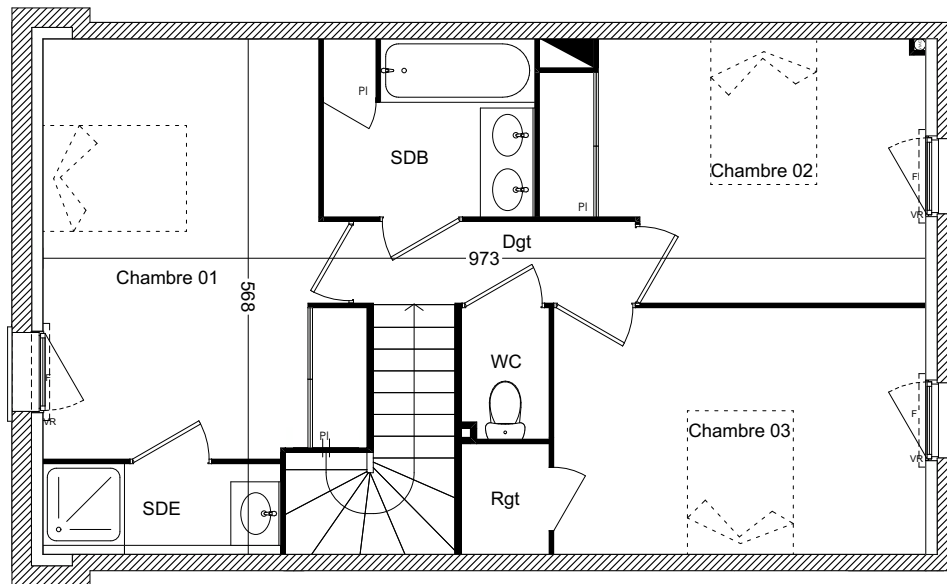
Plan R+1
