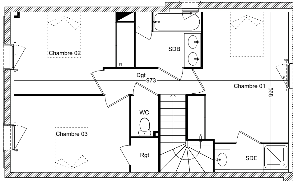
Plan R+1
