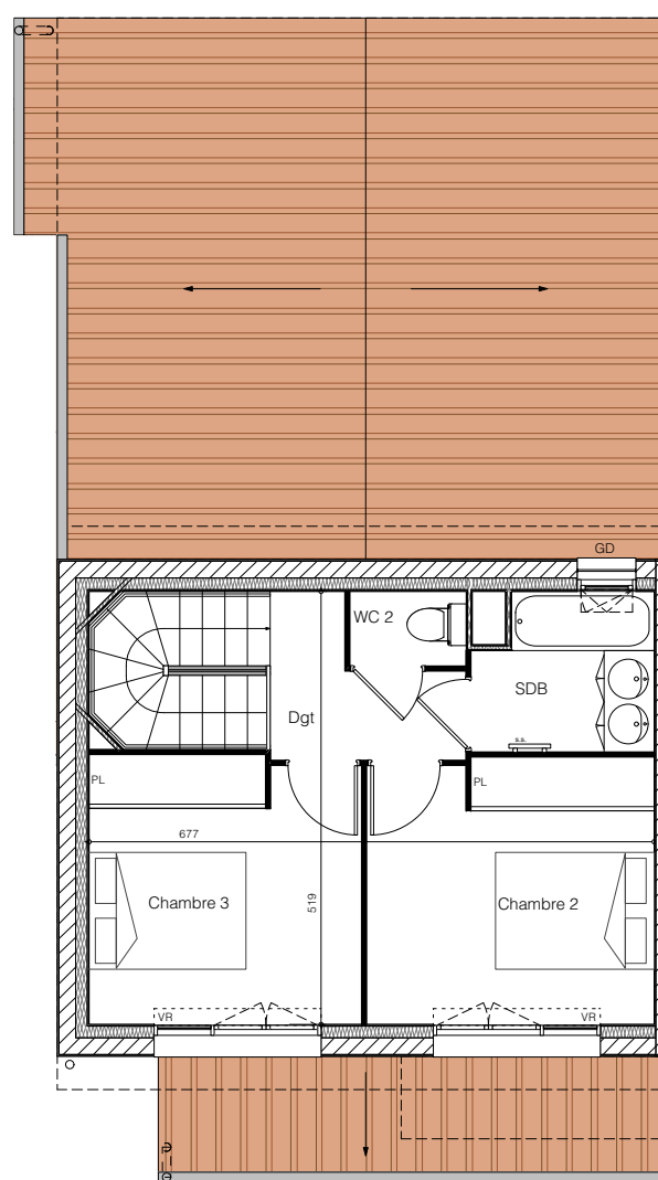
Plan R+1
