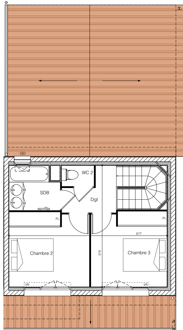
Plan R+1
