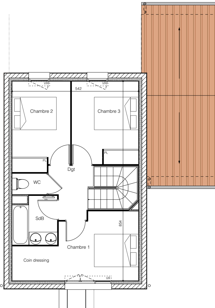
Plan R+1
